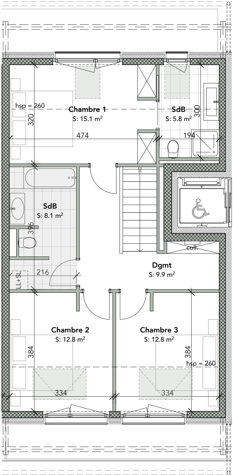
PLAN COMBLES
